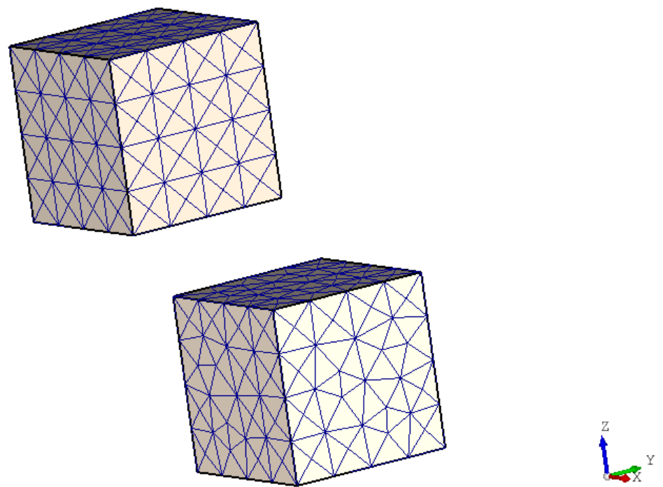
Fig. 3 two different surface grids
